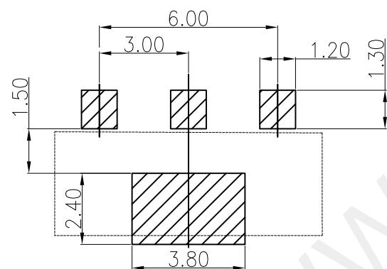
RECOMMENDED PCB LAYOUT TOL:(±0.05)
